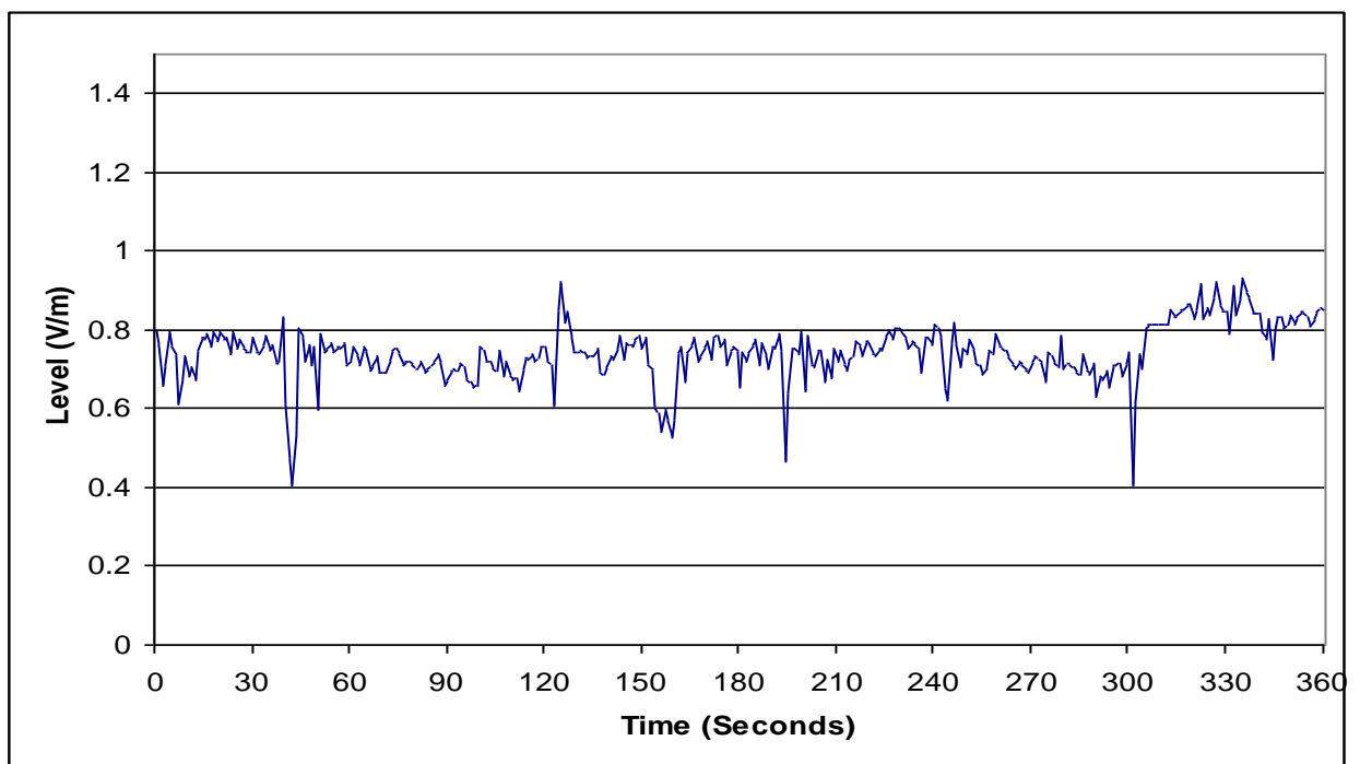
Electric field strengths recorded over 6 min period using 18 GHz probe at point of max NIR:
